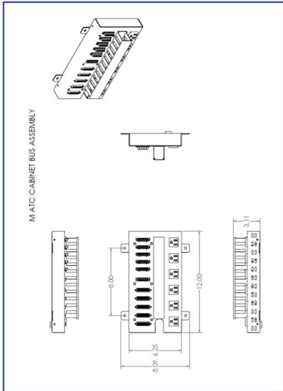
Figure 7: M ATC Cabinet Bus Assembly
